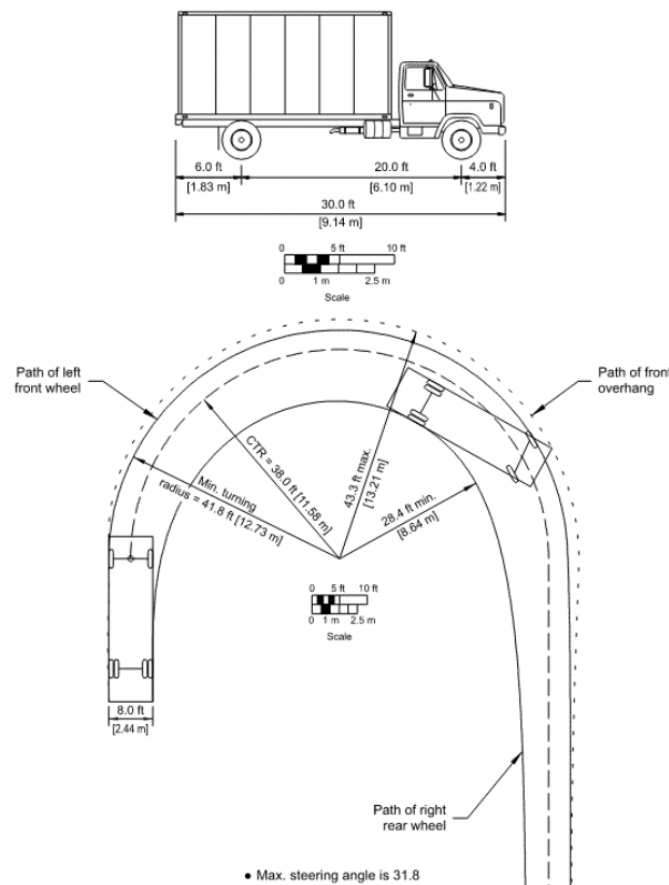
FIGURE B-1* MINIMUM TURNING PATH FOR SU-30 DESIGN VEHICLE
