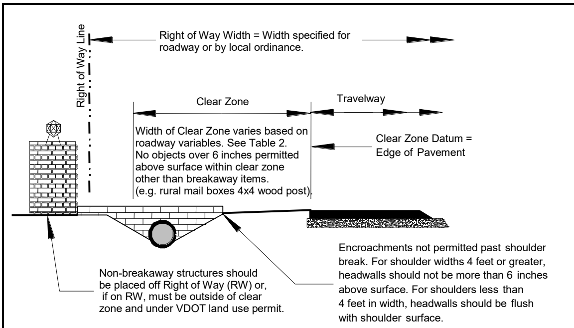
FIGURE B-11* SETBACK DETAILS WITH SHOULDER AND DITCH
