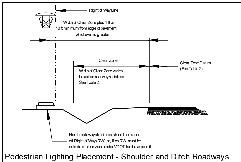
FIGURE B-14* LIGHTING ALONG SHOULDER AND DITCH SECTIONS
