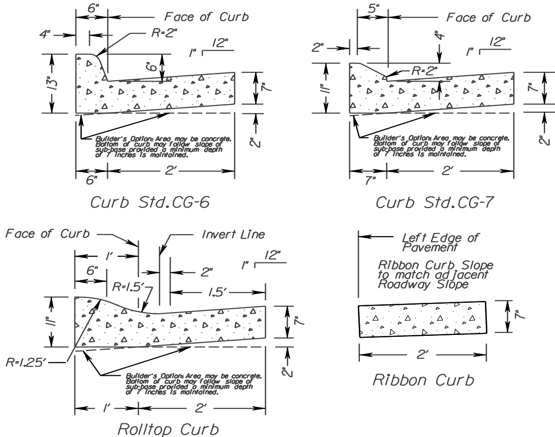
FIGURE B-5* CURB AND GUTTER DETAILS
