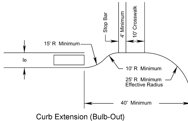
FIGURE B-15** CURB EXTENSION (BULB-OUTS) DETAIL
