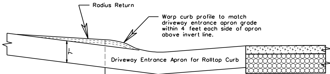
Part Plan of Entrance Transition FIGURE B-7* ROLL TOP CURB ENTRANCE DETAIL
