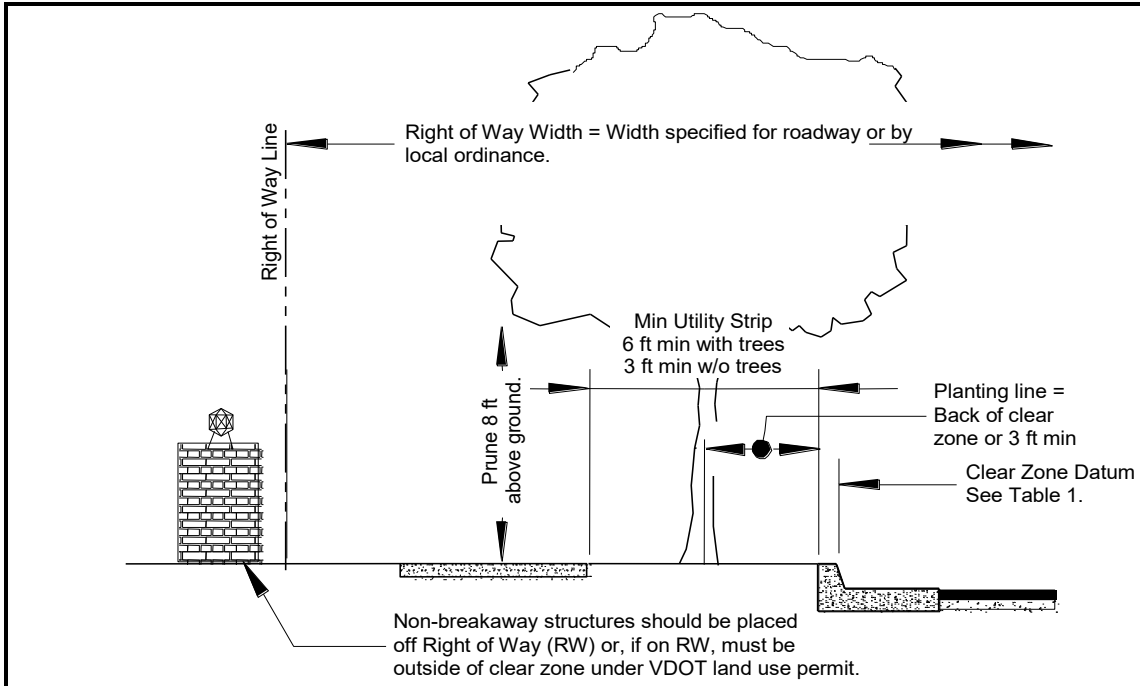
FIGURE B-10* SETBACK DETAILS WITH CURB AND GUTTER
