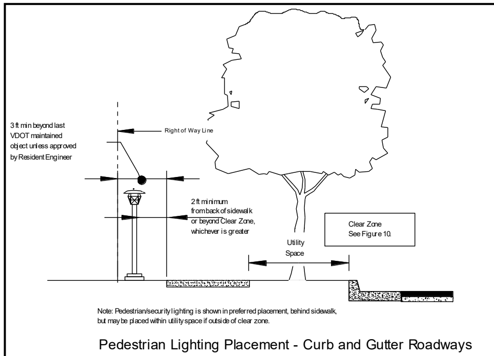
FIGURE B-13* LIGHTING ALONG CURB AND GUTTER SECTIONS
