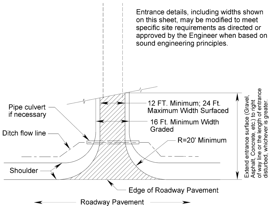
FIGURE B-9* PRIVATE ENTRANCE DETAIL
