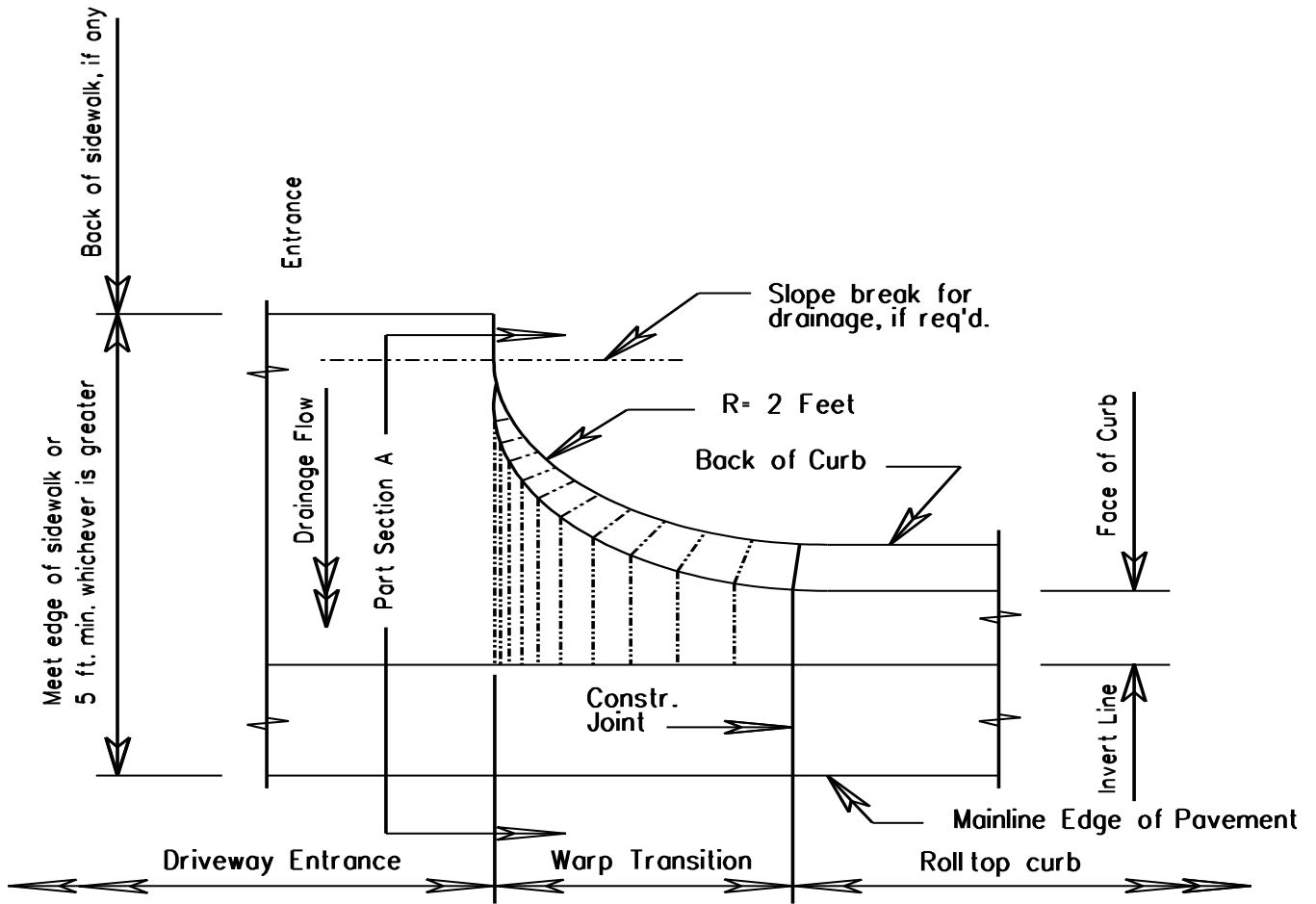
Part Plan of Entrance Transition FIGURE B-7* ROLL TOP CURB ENTRANCE DETAIL
