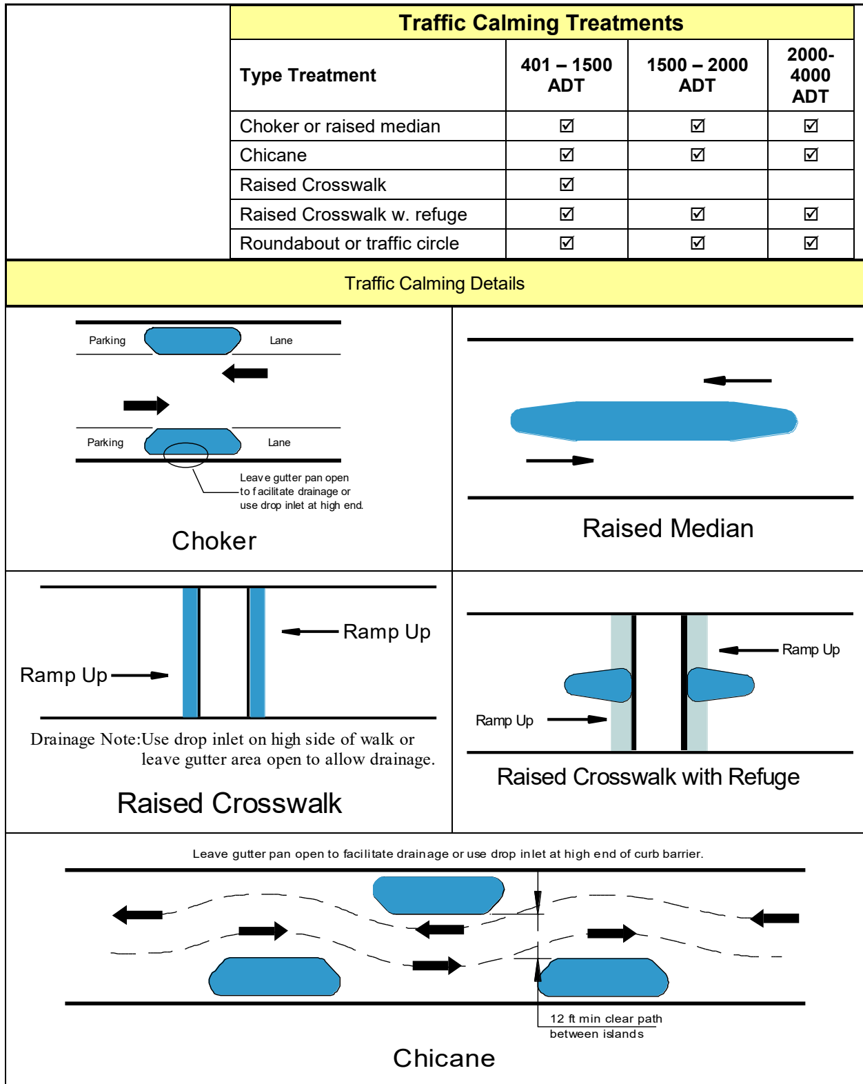
FIGURE B-12* TRAFFIC CALMING DETAILS
