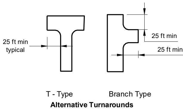
FIGURE B-4* CUL-DE-SAC DETAILS
