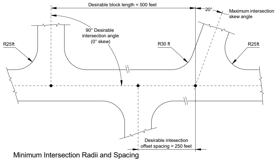
FIGURE B-3 INTERSECTION DESIGN
