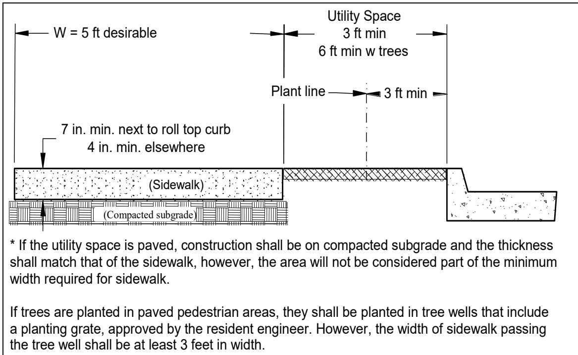
FIGURE B-6* BACK OF CURB DETAILS
